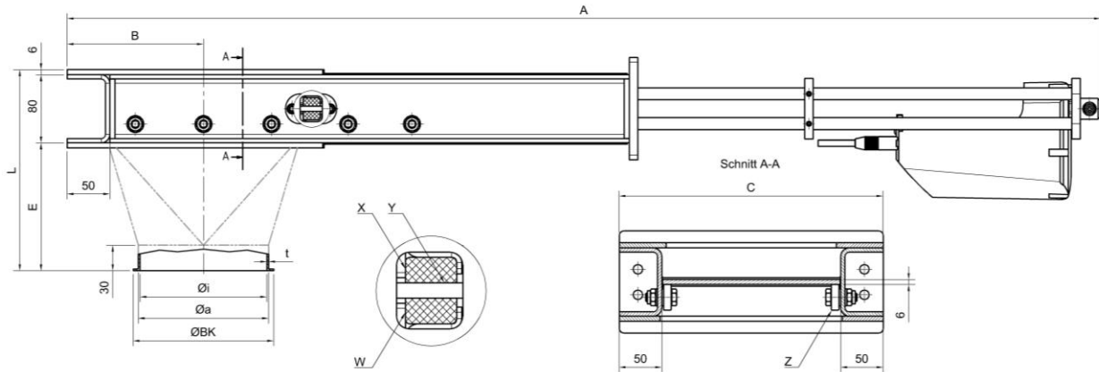
Dimensions Table Silo outlet gate
