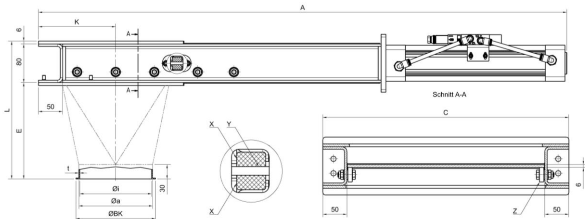
Dimension table Redler outlet gate
